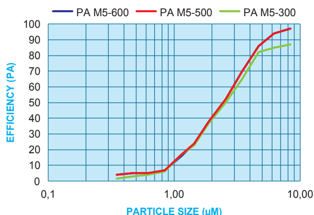
EFFICIENCY vs PARTICLE SIZE
