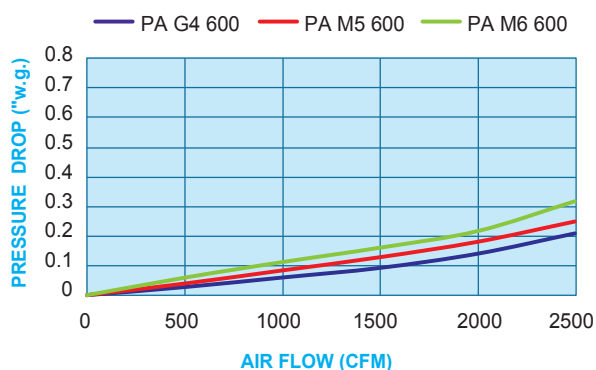
PRESSURE DROP vs AIR FLOW
